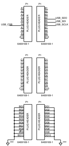
FIFO5 CONNECTIONS
