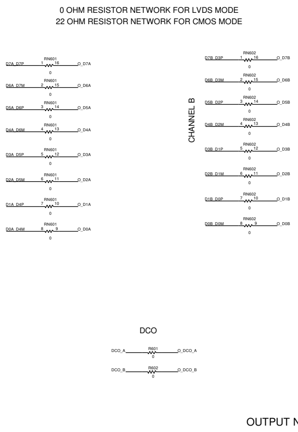
CHANNEL A CHANNEL B Figure 18. Output Buffer Circuits
