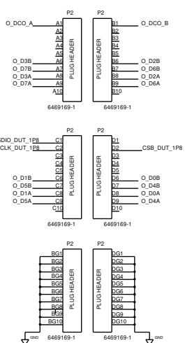
Figure 19. FIFO Board Connector
