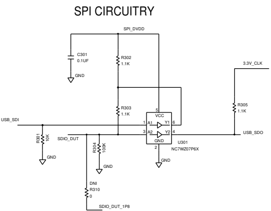
Figure 15. SPI Interface Circuit
