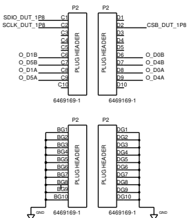
Figure 19. FIFO Board Connector
