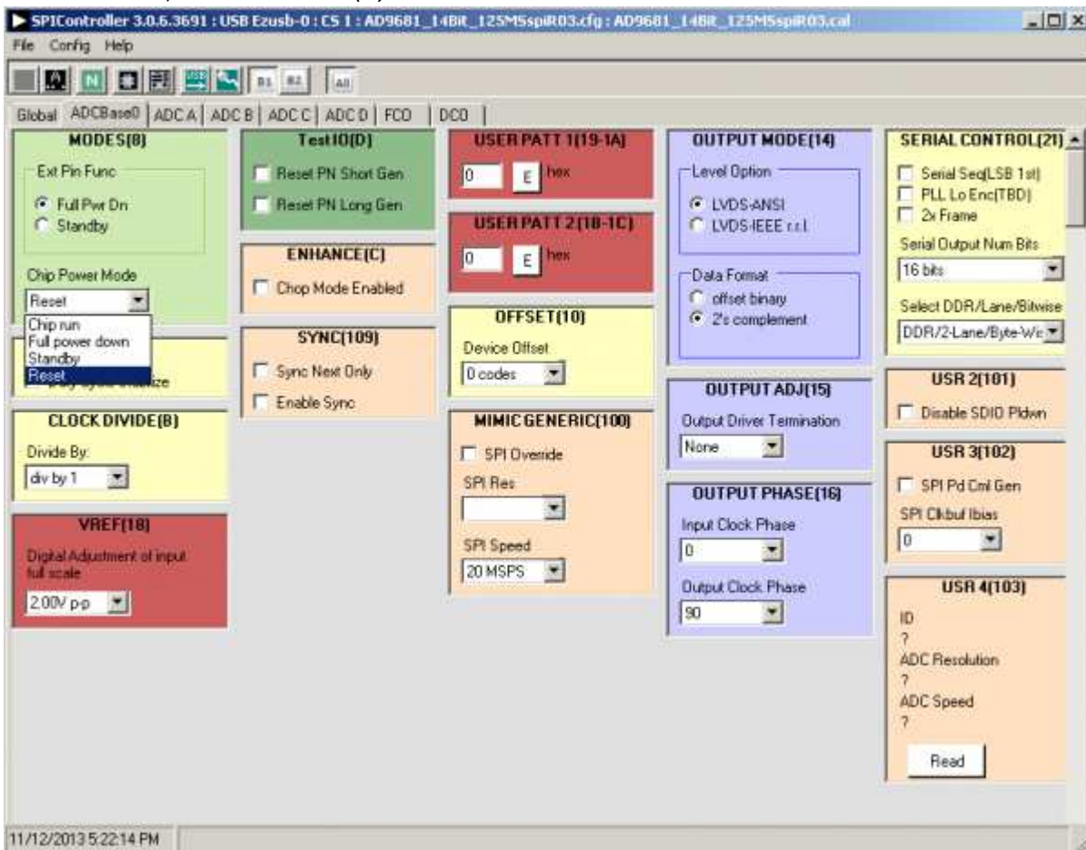
SPI Controller, CLOCK DIVIDE(B) Box
