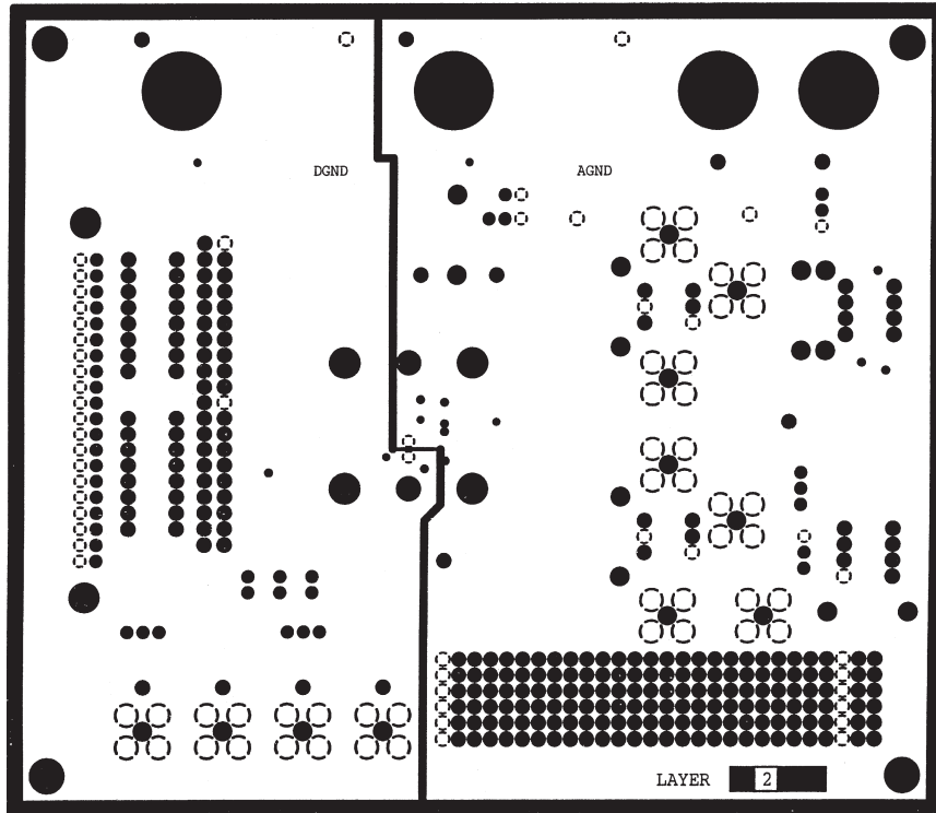
Figure 27. Ground Plane PCB Layout (Layer 2)
