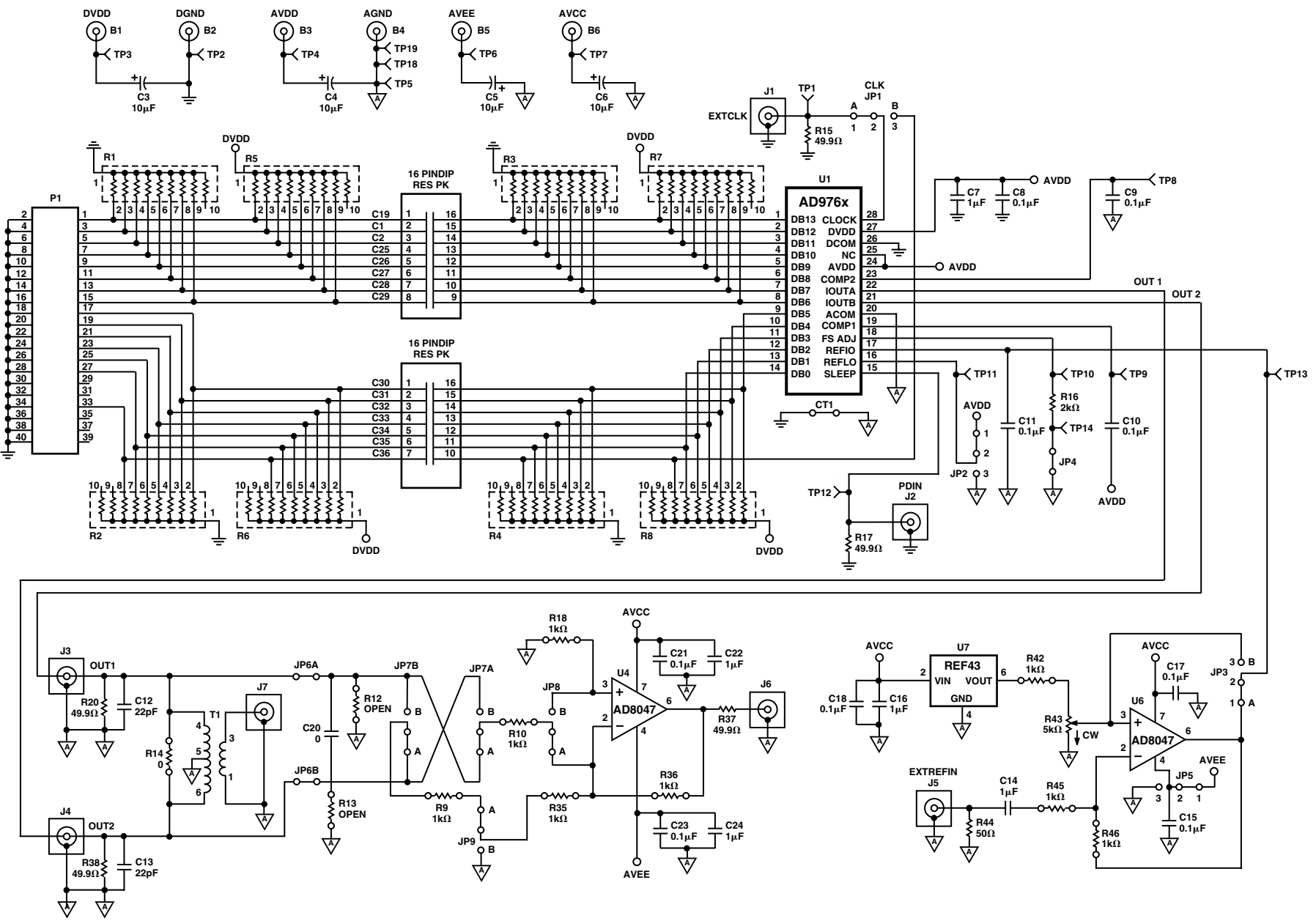
Figure 59. AD9762 Evaluation Board Schematic
