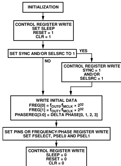
Figure 25. Initialization
