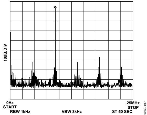
Figure 17. f_{MCLK} = 50 \text{ MHz} , f_{OUT} = 9.1 \text{ MHz} . Frequency Word = 2E978D50
