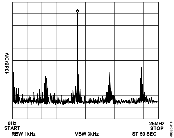
Figure 18. f_{MCLK} = 50 \text{ MHz} , f_{OUT} = 11.1 \text{ MHz} . Frequency Word = 38D4FDF4
