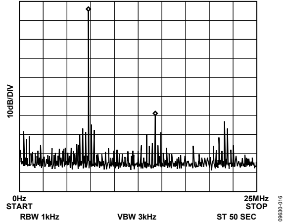
Figure 16. f_{MCLK} = 50 \text{ MHz} , f_{OUT} = 7.1 \text{ MHz} . Frequency Word = 245AICAC
