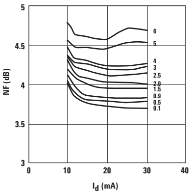
Figure 15. NF vs. I d and Frequency (GHz).
