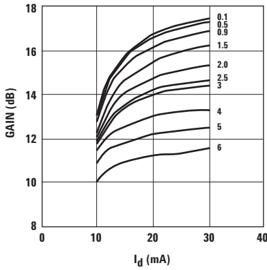
Figure 12. Gain vs. I d and Frequency (GHz).
