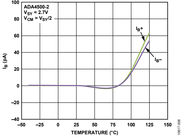
Figure 11. Input Bias Current ( I b ) vs. Temperature, V SY = 2.7 V
