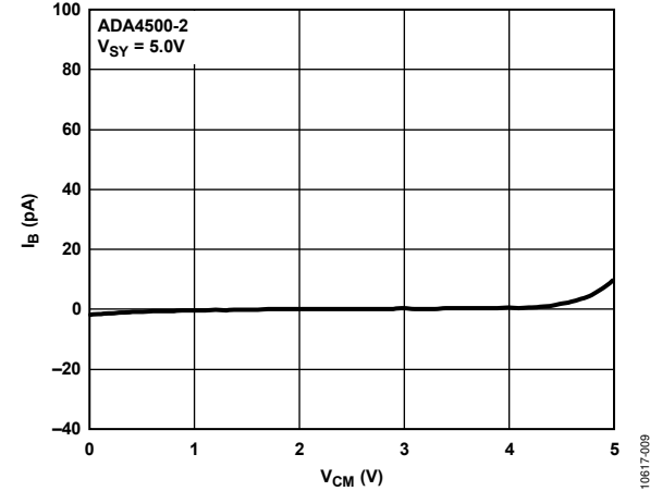
Figure 15. Input Bias Current ( I b ) vs. Common-Mode Voltage ( V CM ), V SY = 5.0 V
