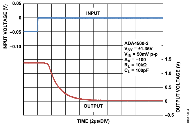
Figure 41. Positive Overload Recovery, V SY = ±1.35 V
