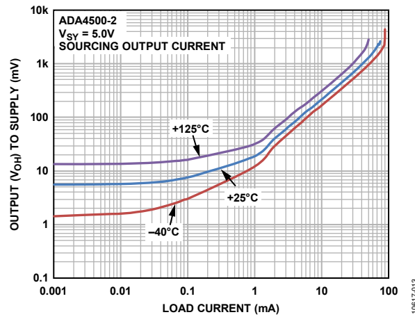
Figure 16. Output Voltage ( V OH ) to Supply Rail vs. Load Current, V SY = 5.0 V
