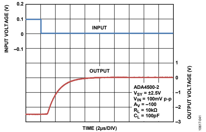
Figure 44. Negative Overload Recovery, V SY = ±2.5 V
