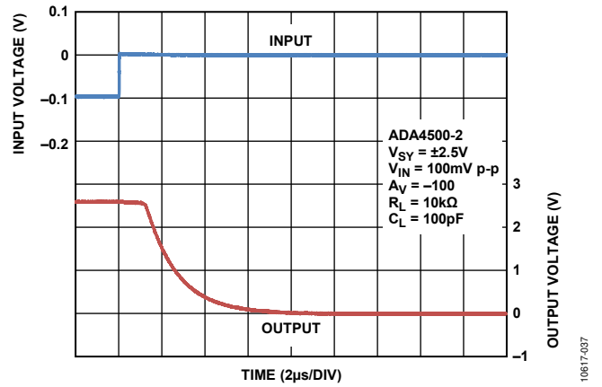
Figure 43. Positive Overload Recovery, V SY = ±2.5 V
