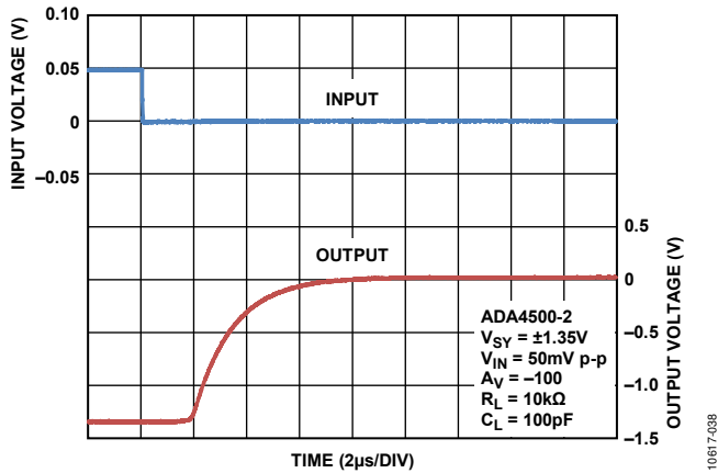
Figure 42. Negative Overload Recovery, V SY = ±1.35 V
