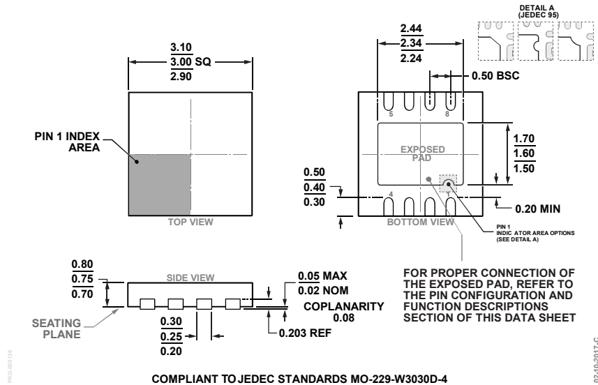
Figure 67. 8-Lead Lead Frame Chip Scale Package [LFCSP] 3 mm x 3 mm Body and 0.75 mm Package Height (CP-8-11) Dimensions shown in millimeters
