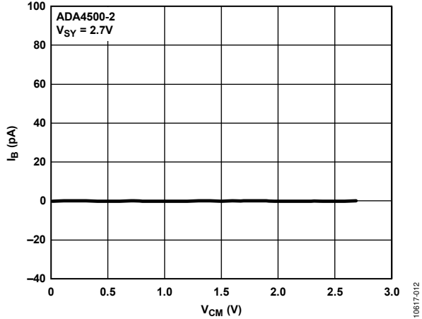
Figure 12. Input Bias Current ( I b ) vs. Common-Mode Voltage ( V CM ), V SY = 2.7 V
