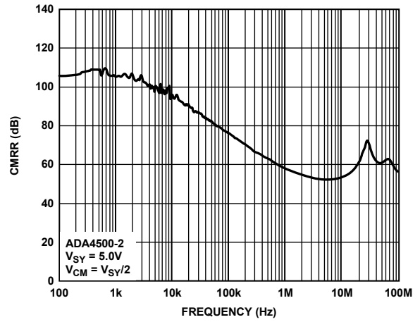
Figure 32. CMRR vs. Frequency, V SY = 5.0 V
