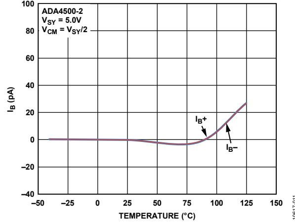
Figure 14. Input Bias Current ( I b ) vs. Temperature, V SY = 5.0 V
