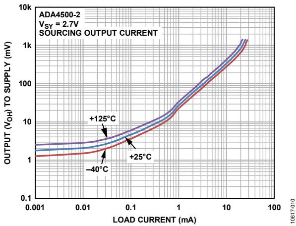
Figure 13. Output Voltage ( V OH ) to Supply Rail vs. Load Current, V SY = 2.7 V
