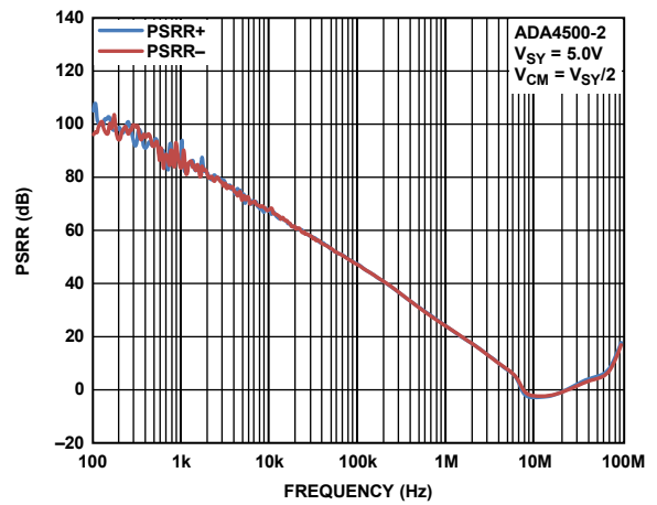
Figure 33. PSRR vs. Frequency, V SY = 5.0 V
