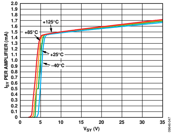
Figure 52. Supply Current ( I_{SV} ) per Amplifier vs. Supply Voltage ( V_{SV} ) at Various Temperatures
