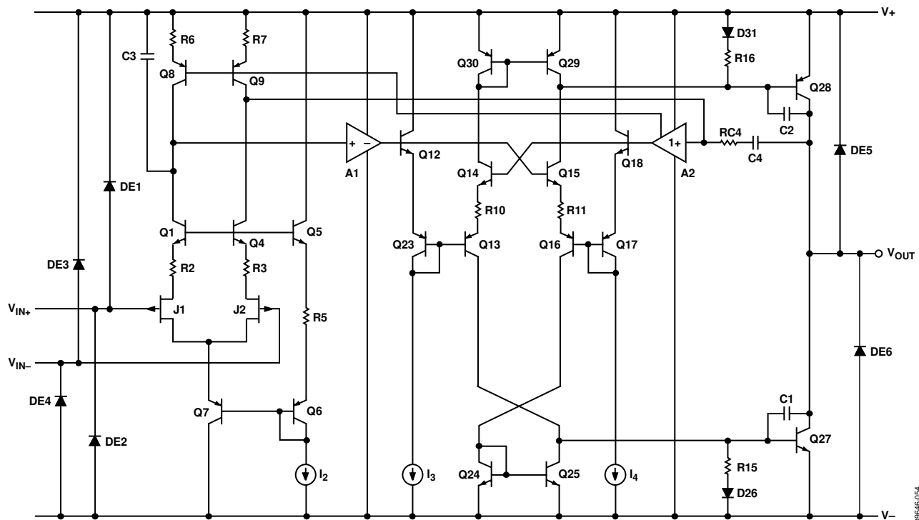
Figure 57. Simplified Schematic
