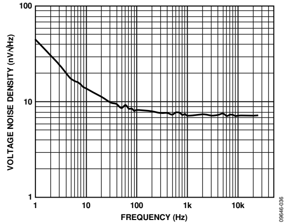
Figure 41. Voltage Noise Density vs. Frequency, V_{SV} = \pm 15 V
