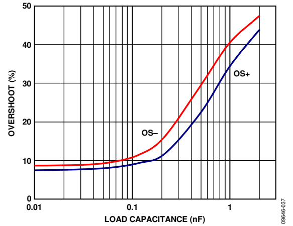
Figure 42. Overshoot vs. Load Capacitance, V_{SV} = \pm 15 V , A_V = +1 , R_L = 2 k\Omega , V_{IN} = 100 mV p-p
