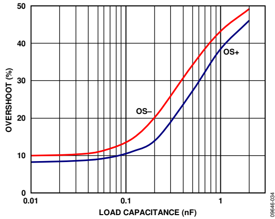
Figure 40. Overshoot vs. Load Capacitance, V_{SV} = \pm 5 V , A_V = +1 , R_L = 2 k\Omega , V_{IN} = 100 mV p-p
