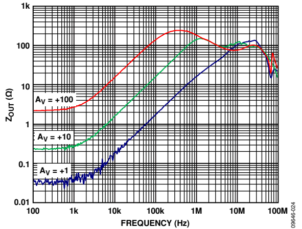
Figure 31. Closed-Loop Output Impedance ( Z_{OUT} ) vs. Frequency, V_{SV} = \pm 15 V
