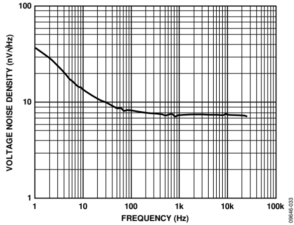
Figure 39. Voltage Noise Density vs. Frequency, V_{SV} = \pm 5 V
