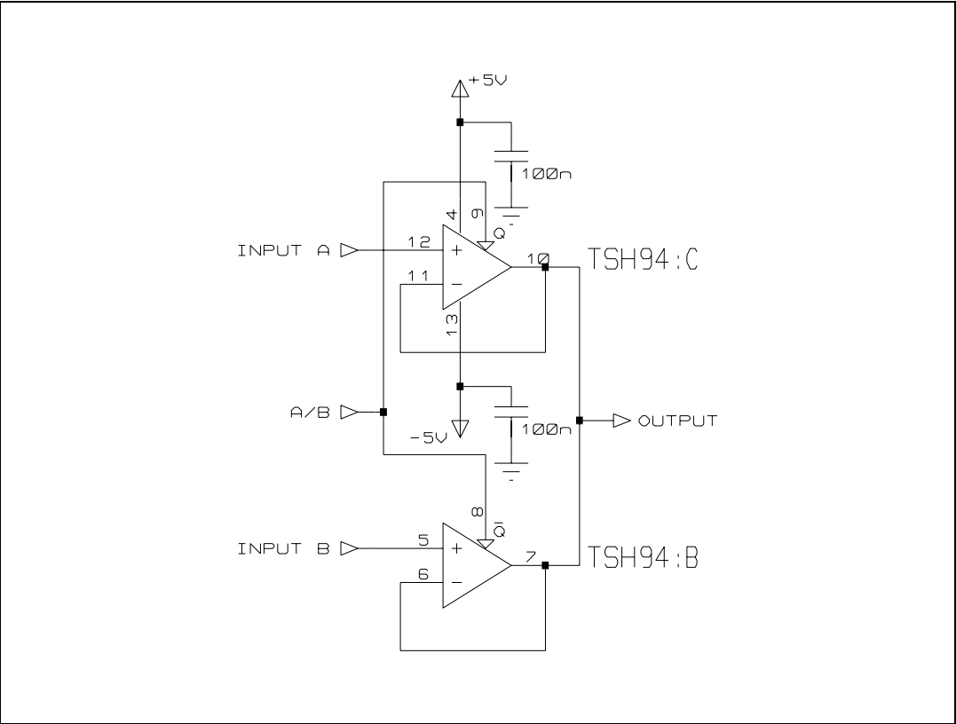
Figure 18. Signal multiplexing
