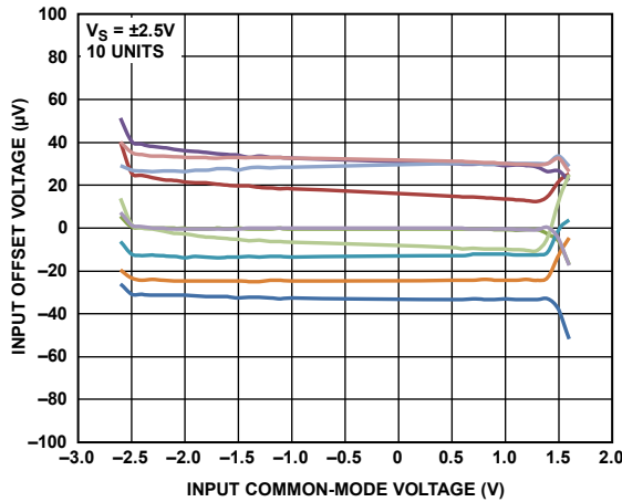
Figure 27. Input Offset Voltage vs. Input Common-Mode Voltage
