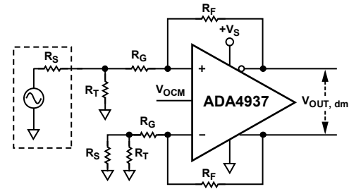
Figure 55. ADA4937-1/ADA4937-2 Configured for Unbalanced (Single-Ended) Input
