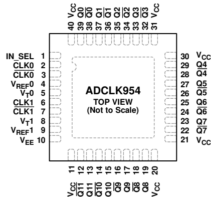
Figure 2. Pin Configuration
