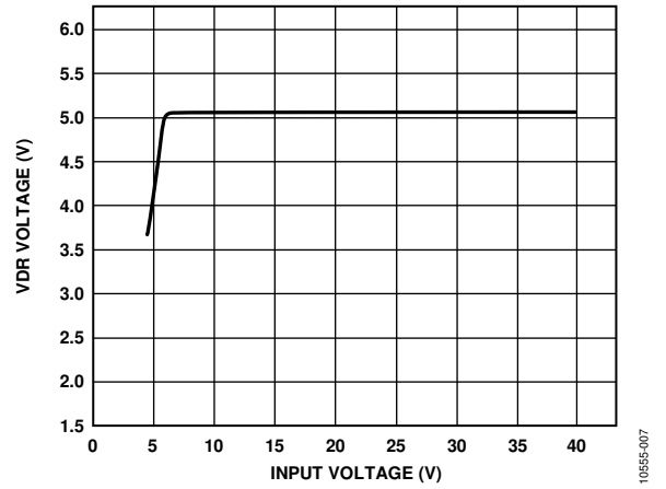
Figure 8. VDR Voltage vs. Input Voltage
