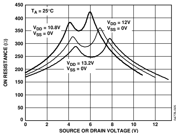
Figure 6. On Resistance as a Function of V_D ( V_S ) for Single Supply
