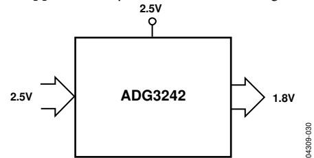
Figure 31. 2.5 V to 1.8 V Voltage Translation, \overline{SEL} = 2.5\text{ V}
