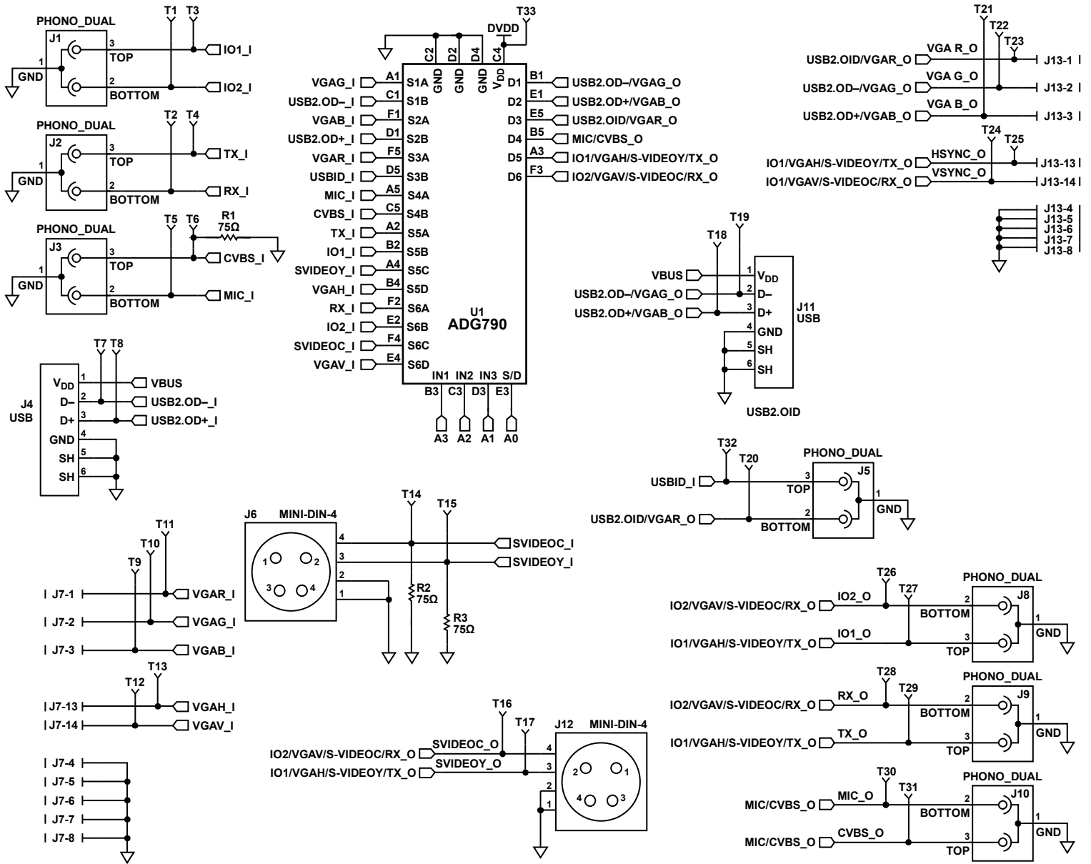
Figure 28. EVAL-ADG790 Schematic Switch Section
