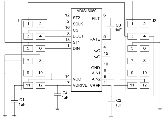
Figure 1 - ADIS16080/PCB Schematic
