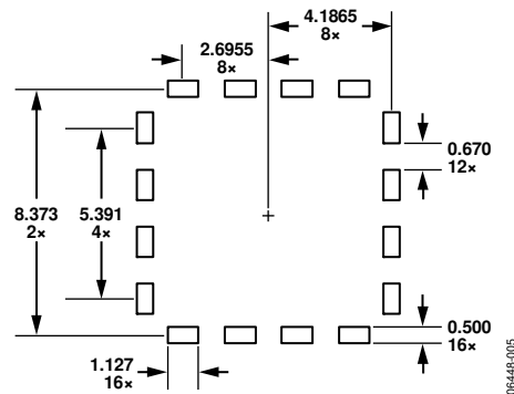
9.2mm x 9.2mm STACKED LGA PACKAGE
