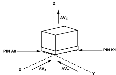
Figure 36. Delta Velocity Axis and Polarity Assignments
