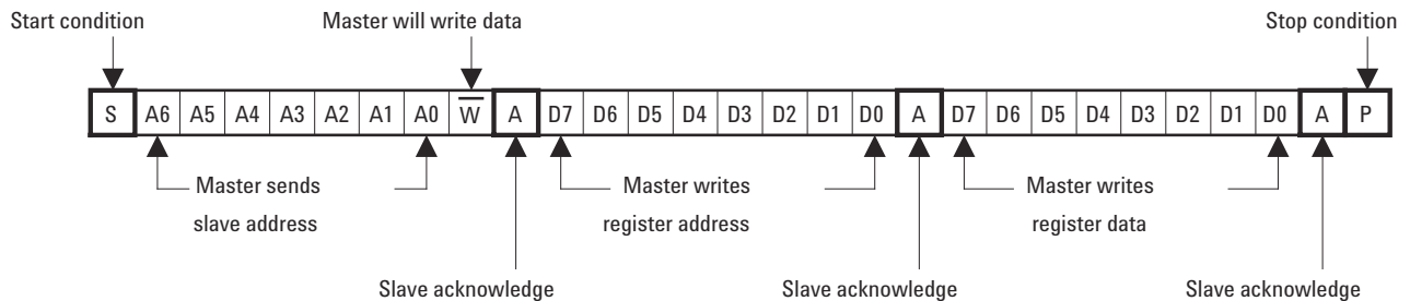
Figure 9. Register Byte Write Protocol
