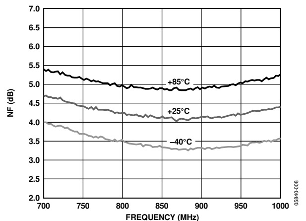
Figure 9. Noise Figure vs. Frequency and Temperature, 800 MHz to 960 MHz
