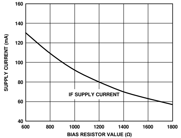
Figure 41. IF Supply Current vs. IF Bias Resistor Value
