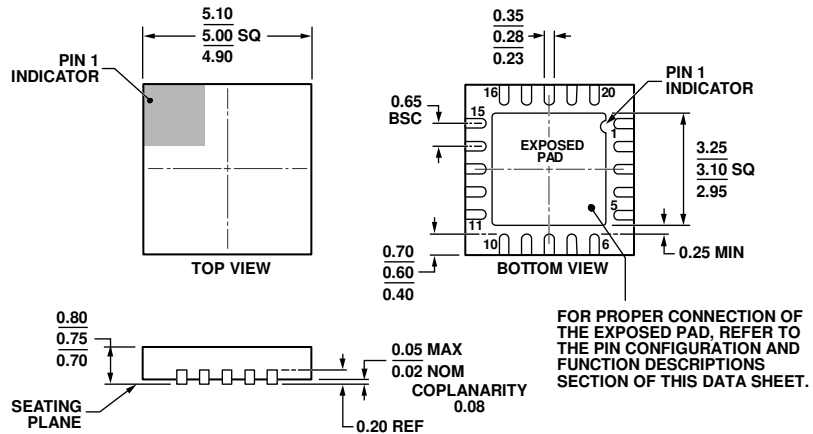
Figure 57. 20-Lead Lead Frame Chip Scale Package [LFCSP_WQ] 5 mm x 5 mm Body, Very Very Thin Quad (CP-20-9) Dimensions shown in millimeters
