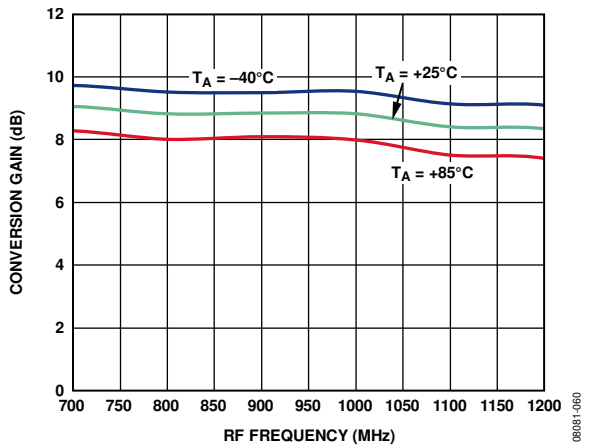
Figure 45. Power Conversion Gain vs. RF Frequency at 3.3 V
