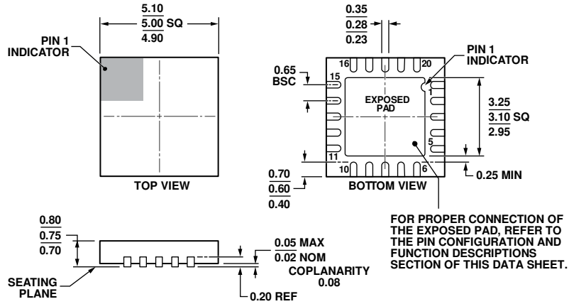
Figure 57. 20-Lead Lead Frame Chip Scale Package [LFCSP_WQ] 5 mm × 5 mm Body, Very Very Thin Quad (CP-20-9) Dimensions shown in millimeters
