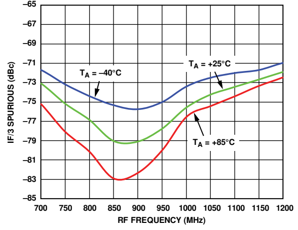
Figure 26. IF/3 Spurious vs. RF Frequency
