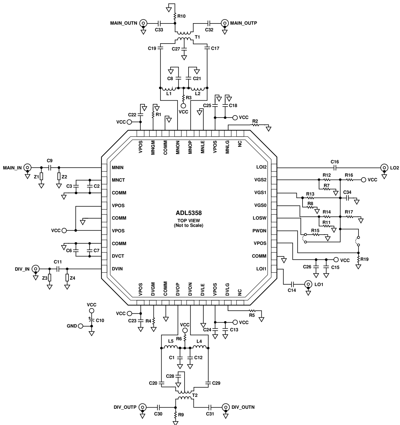
Figure 54. Evaluation Board Schematic
