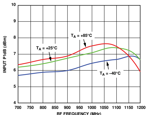
Figure 50. Input P1dB vs. RF Frequency at 3.3 V
