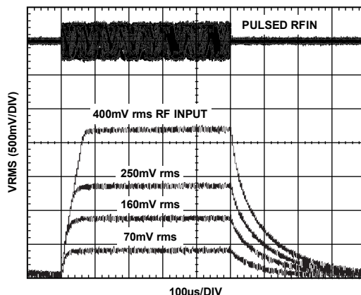
Figure 33. Output Response to Various RF Input Pulse Levels, Supply = 3 V, Frequency = 900 MHz, C_{FLTR} = \text{Open} , C_{OUT} = 0.1\text{ µF} , R_{OUT} = 1\text{ k}\Omega
