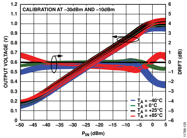
Figure 25. Distribution of Log Conformance Error with Respect to V_{LOG} at 25^\circ\text{C} vs. P_{IN} and Temperature at 2700 MHz
