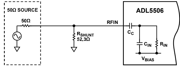
Figure 46. Broadband Resistive Method for Input Coupling
