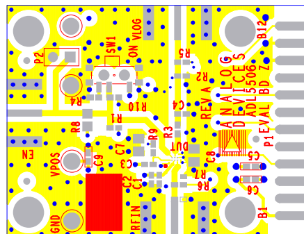
Figure 52. Layout of Evaluation Board, Component Side
