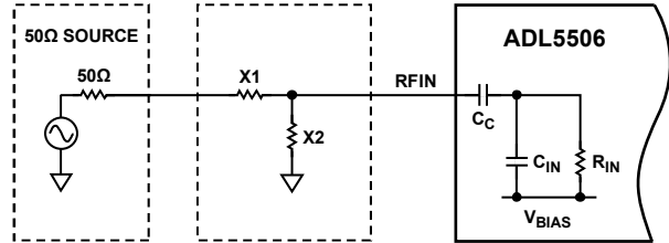
Figure 47. Narrow-Band Reactive Method for Input Coupling
