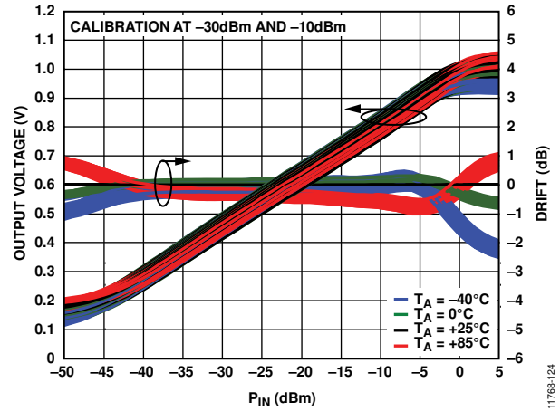
Figure 24. Distribution of Log Conformance Error with Respect to V_{LOG} at 25^\circ\text{C} vs. P_{IN} and Temperature at 2140 MHz
