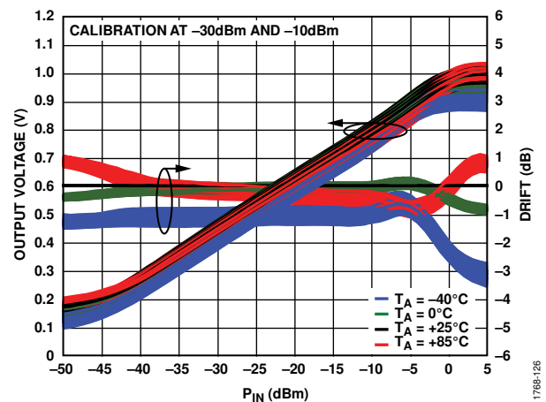
Figure 26. Distribution of Log Conformance Error with Respect to V_{LOG} at 25^\circ\text{C} vs. P_{IN} and Temperature at 3500 MHz
