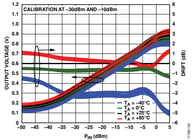
Figure 30. Distribution of Log Conformance Error with Respect to V_{LOG} at 25^\circ\text{C} vs. P_{IN} and Temperature at 4500 MHz
