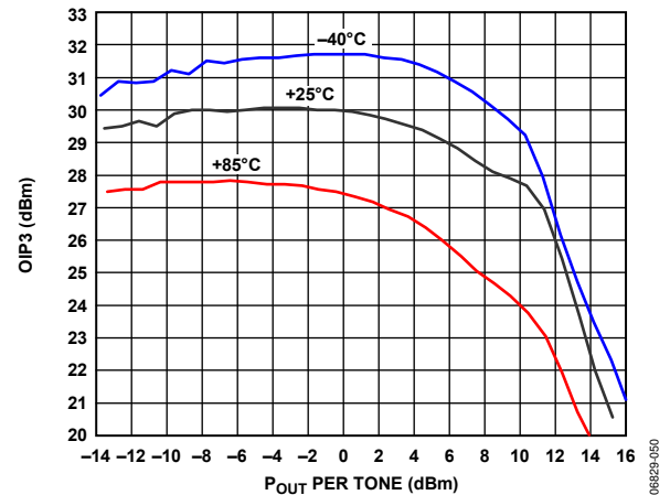
Figure 50. OIP3 vs. Output Power ( P_{OUT} ) and Temperature
