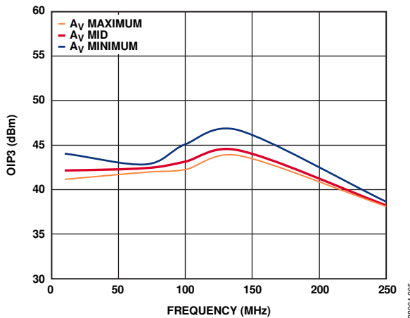
Figure 11. OIP3 vs. Frequency (Single-Ended Input)
