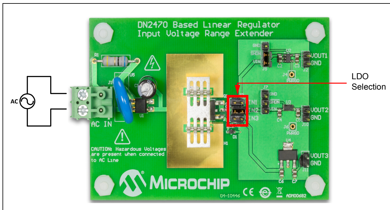
FIGURE 2-1: DN2470 Based Linear Regulator Input Voltage Range Extender Evaluation Board.
