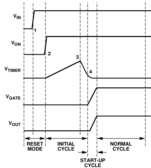
Figure 33. Power-Up Timing
