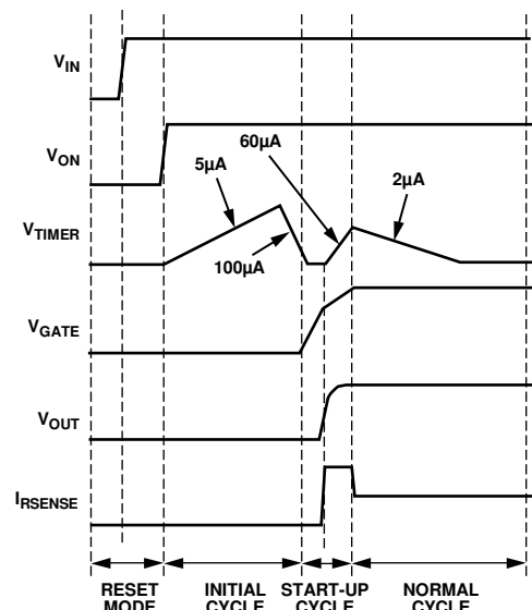
Figure 37. Power-Up into Capacitor
