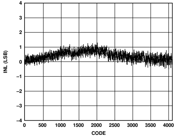
Figure 28. INL for ADC
