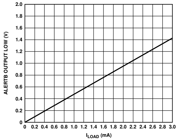
Figure 32. ALERTB Output Low Voltage vs. Load Current
