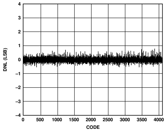
Figure 29. DNL for ADC
