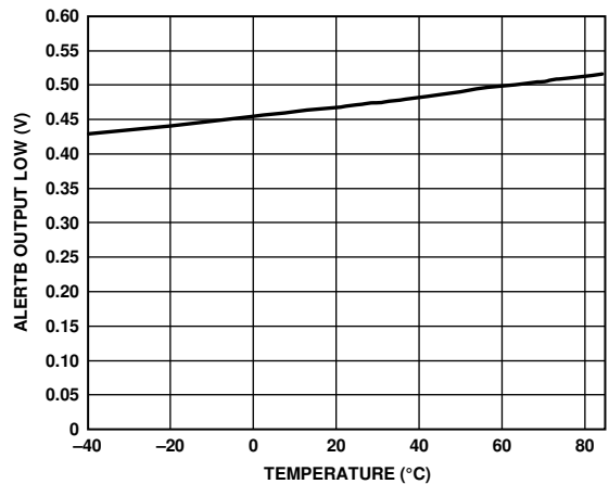
Figure 30. ALERTB Output Low Voltage vs. Temperature @ 1 mA
