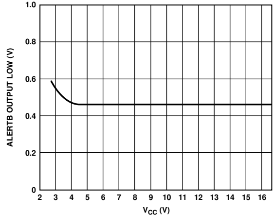
Figure 31. ALERTB Output Low Voltage vs. Supply @ 1 mA
