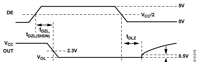
Figure 19. Driver Enable and Disable Times ( t_{DZL} , t_{DZL(SHDN)} , t_{DZH} , t_{DZH(SHDN)} , t_{DHL} )
