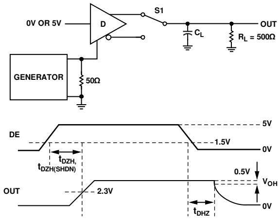
Figure 21. Driver Enable and Disable Times ( t_{DZH} , t_{DZH(SHDN)} , t_{DHL} , t_{DHL(SHDN)} )
