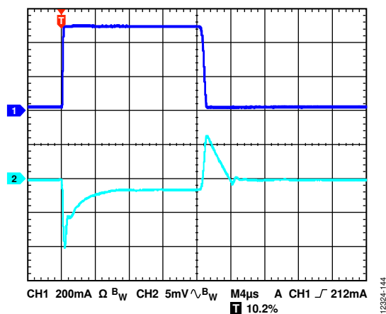
Figure 44. Output Transient Response, V_{OUT} = 3.3\text{ V} , C_{OUT} = 10\ \mu\text{F} , CH1 = \text{Load Current} , CH2 = V_{OUT}
