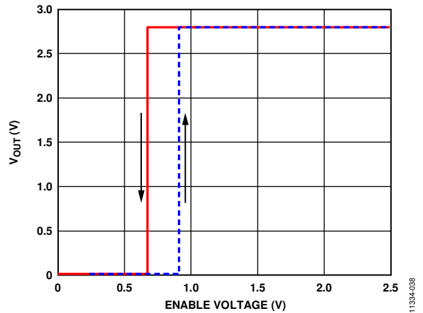
Figure 36. Typical EN Pin Operation
