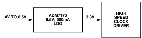
Figure 67. Clock Driver
