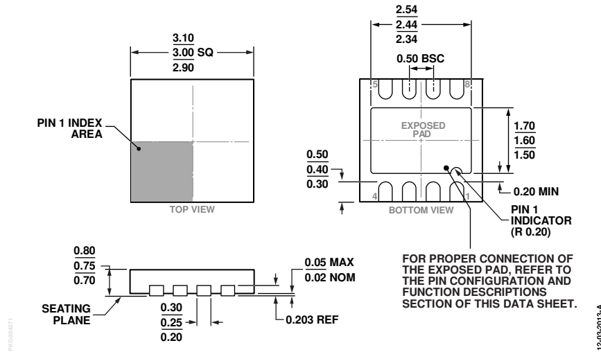
Figure 70. 8-Lead Lead Frame Chip Scale Package [LFCSP_WD] 3 mm x 3 mm Body, Very Very Thin, Dual Lead (CP-8-21) Dimensions shown in millimeters
