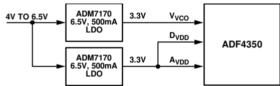
Figure 68. RF PLL/VCO Power
