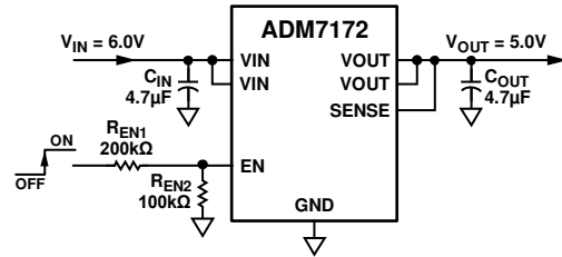
Figure 61. Typical EN Pin Voltage Divider
