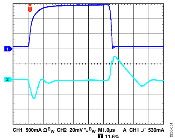
Figure 51. Load Transient Response, I_{LOAD} = 100\text{ mA} to 1.6\text{ A} , Adjustable Version, V_{OUT} = 1.2\text{ V} , V_{IN} = 2.5\text{ V} , CH1 = I_{LOAD} , CH2 = V_{OUT}
