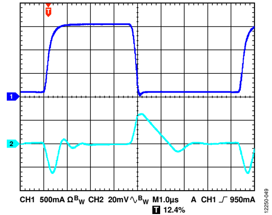
Figure 49. Load Transient Response, I_{LOAD} = 100\text{ mA} to 1.6\text{ A} , V_{OUT} = 5\text{ V} , V_{IN} = 5.5\text{ V} , CH1 = I_{LOAD} , CH2 = V_{OUT}
