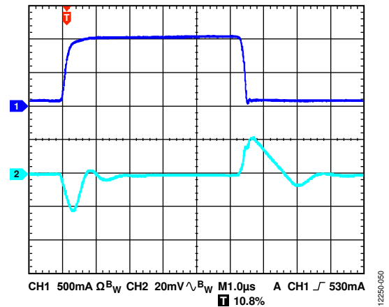
Figure 50. Load Transient Response, I_{LOAD} = 10\text{ mA} to 1\text{ A} , Adjustable Version, V_{OUT} = 1.2\text{ V} , V_{IN} = 2.5\text{ V} , CH1 = I_{LOAD} , CH2 = V_{OUT}
