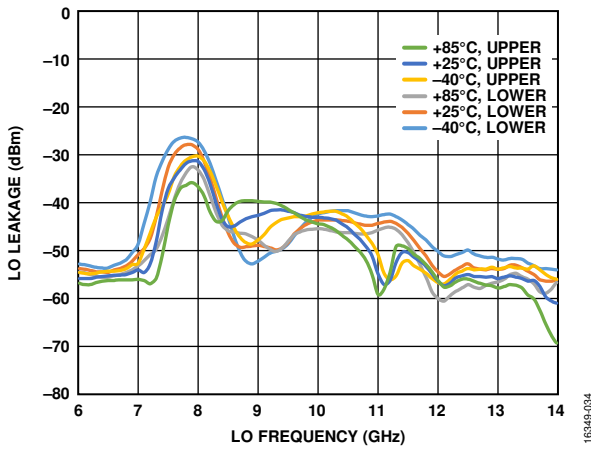
Figure 27. LO Leakage at IF Output vs. LO Frequency at Various Temperatures and Sidebands
