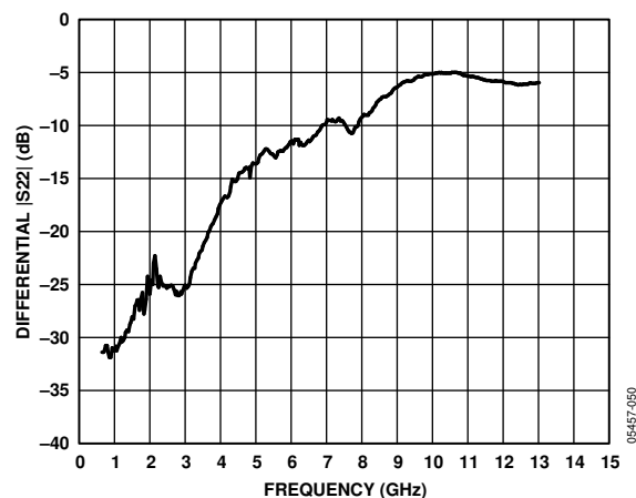
Figure 10. Differential |S22|
