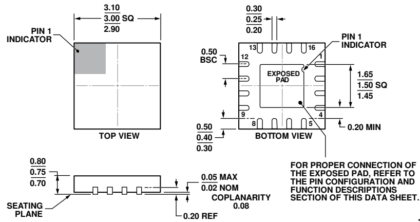
Figure 41. 16-Lead Lead Frame Chip Scale Package [LFCSP_WQ] 3 mm x 3 mm Body, Very Very Thin Quad (CP-16-27) Dimensions shown in millimeters
