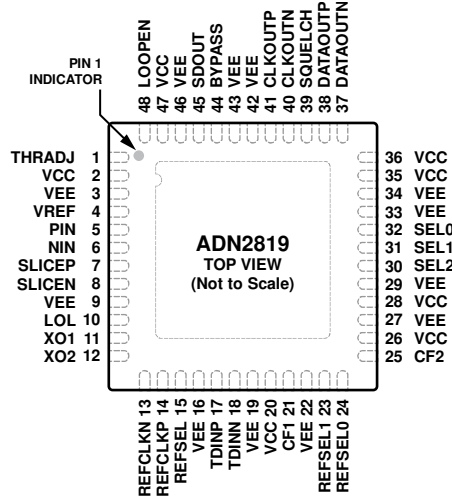
Figure 2. 48-Lead LFCSP Pin Configuration
