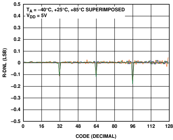
Figure 11. R-DNL—7-Bit RDAC
