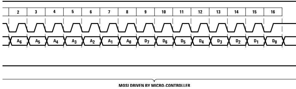
Figure 11. Write operation
