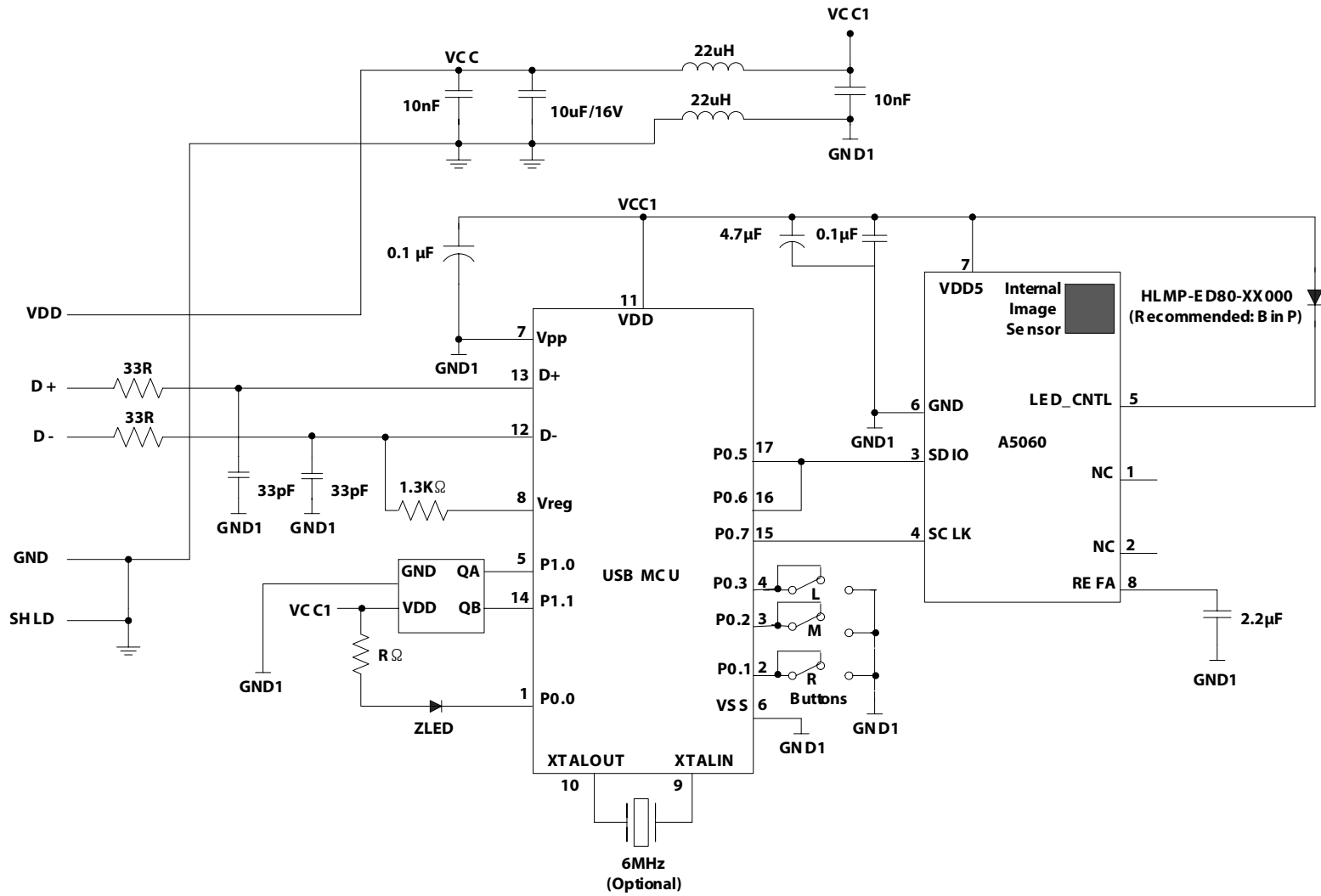
Figure 7b. Schematic Diagram for Interface between ADNS-5060 and Microcontroller (using internal LED driver)
