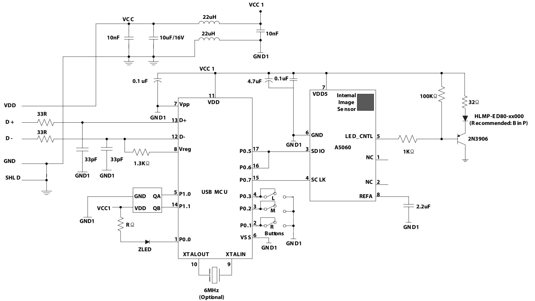
Figure 7a. Schematic Diagram for Interface between ADNS-5060 and Microcontroller (compatible with A26x0 sensors)
