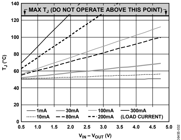
Figure 36. 500 mm 2 of PCB Copper, T_A = 50^\circ\text{C}
