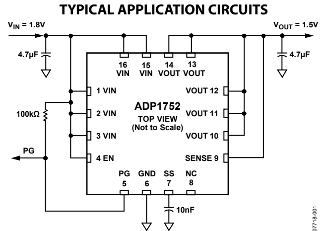
Figure 1. ADP1752 with Fixed Output Voltage, 1.5 V
