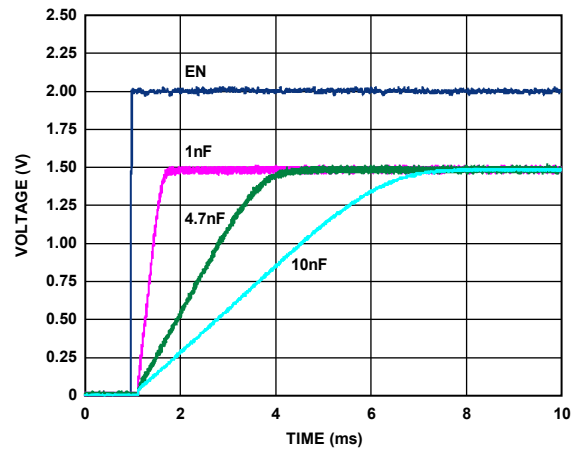
Figure 26. V_{OUT} Ramp-Up with External Soft Start Capacitor
