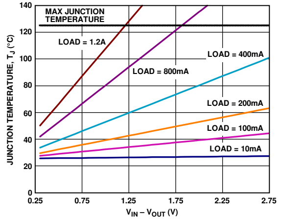
Figure 12. 500 mm 2 of PCB Copper, T_A = 25^\circ\text{C} , LFCSP
