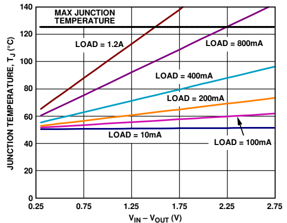
Figure 14. 6400 mm 2 of PCB Copper, T_A = 50^\circ\text{C} , LFCSP
