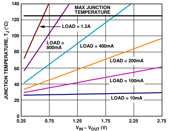
Figure 13. 0 mm 2 of PCB Copper, T_A = 25^\circ\text{C} , LFCSP
