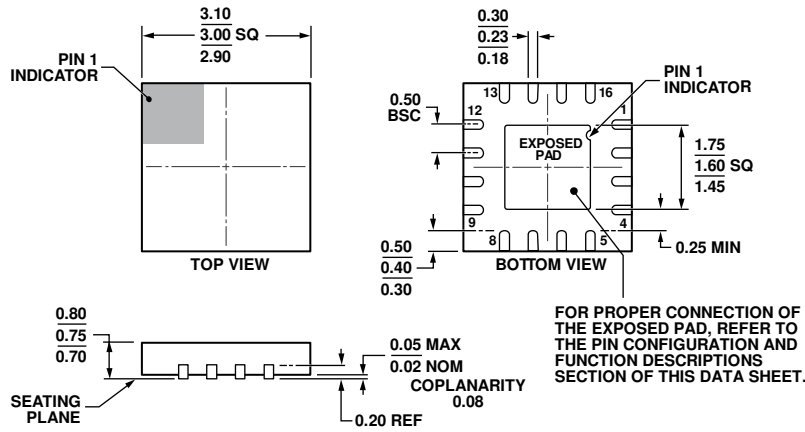
Figure 47. 16-Lead Lead Frame Chip Scale Package [LFCSP] 3 mm × 3 mm Body and 0.75 mm Package Height (CP-16-22) Dimensions shown in millimeters
